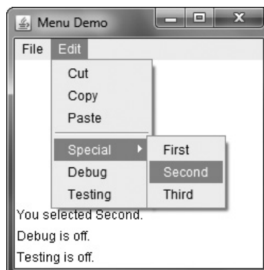
Figure 26-8 Sample output from the MenuDemo applet
