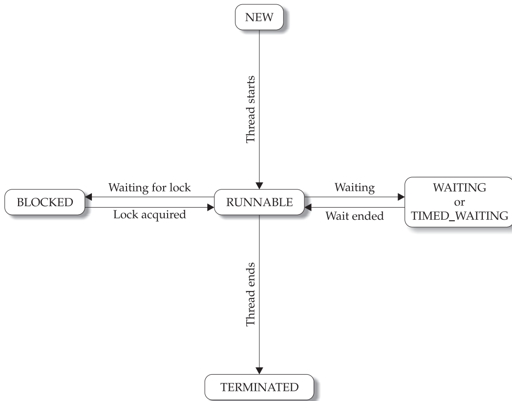
Figure 11-1 Thread states
